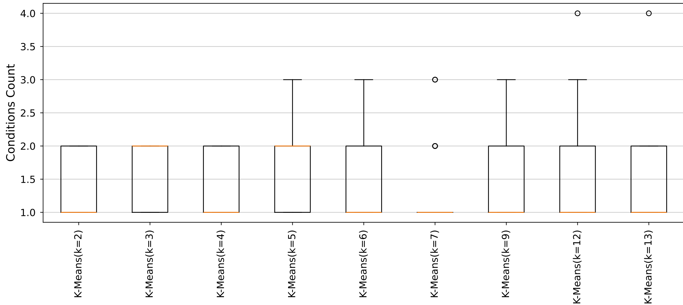
YARA Rules Conditions Count Distribution (Cluster8_Size13 dataset)
